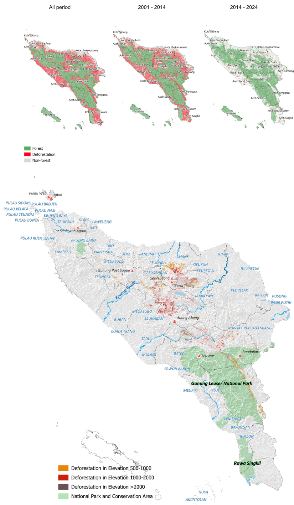
Figure 3.5. Deforestation in Aceh over time and over different elevation. Source: Hansen, M. C., P. V. Potapov, R. Moore, M. Hancher, S. A. Turubanova, A. Tyukavina, D. Thau, S. V. Stehman, S. J. Goetz, T. R. Loveland, A. Kommareddy, A. Egorov, L. Chini, C. O. Justice, and J. R. G. Townshend. 2013. "High-Resolution Global Maps of 21st-Century Forest Cover Change." Science 342 (15 November): 850-853.
